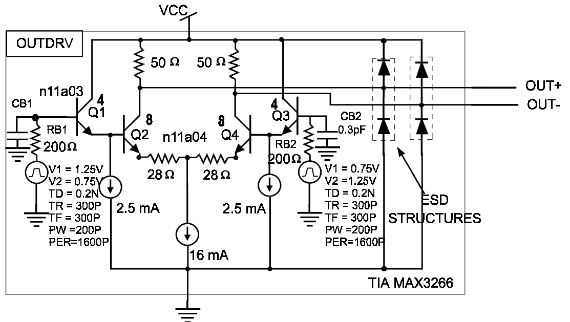
Figure 1. Output signal buffer for the MAX3266 used in dice form. For bondwires estimate 0.9nH/mm and 0.04Ohms/mm.
