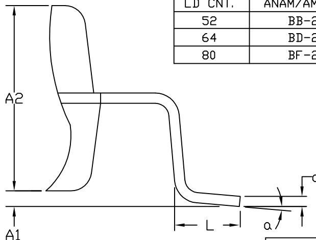
DETAIL "B"
