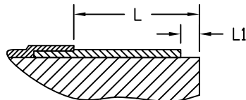
SECTION A-A SCALE 5:1
