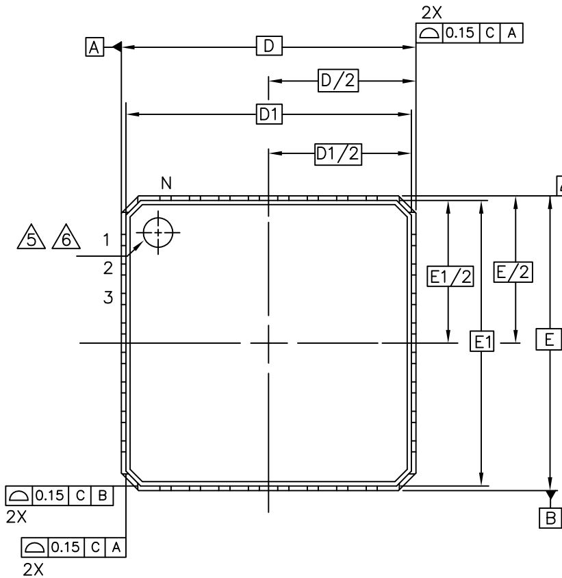
TOP VIEW
