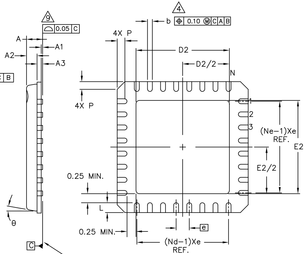
SIDE VIEW
