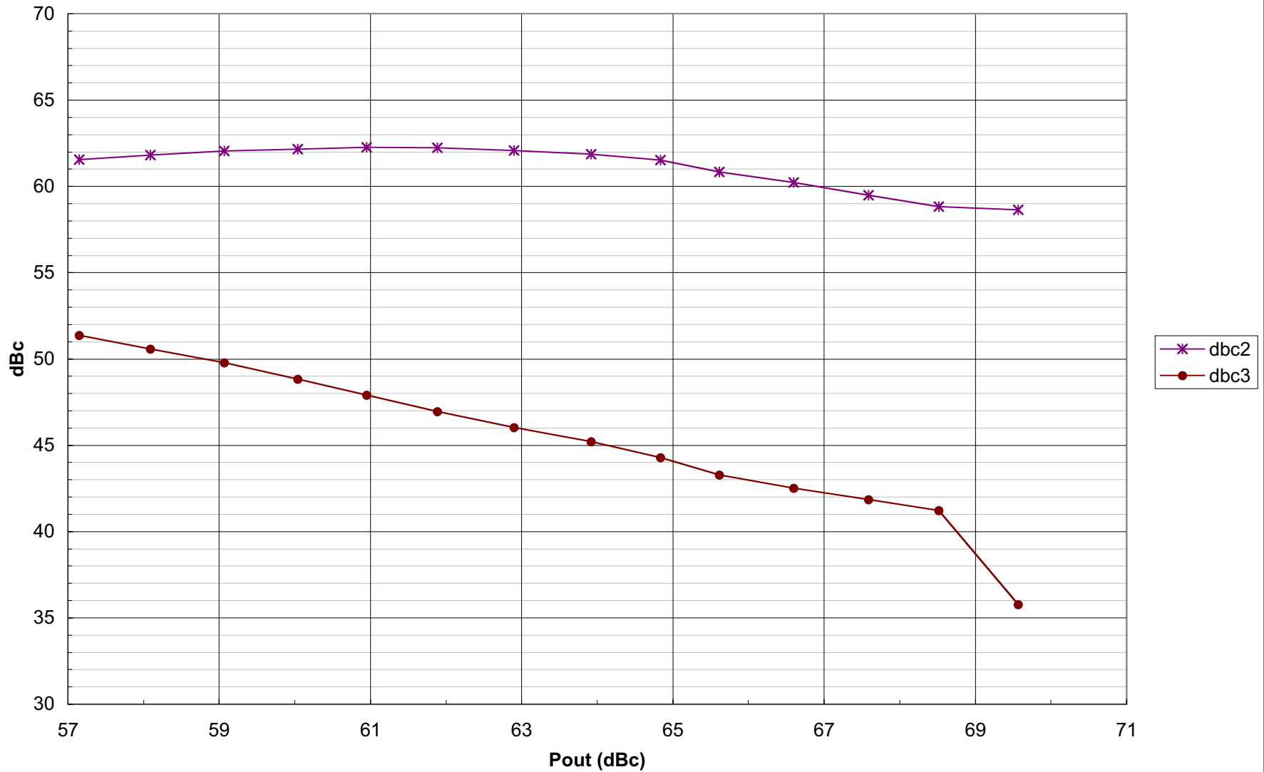
2nd 3rd Harmonic vs. Pout MAX3509 65MHz 2:1 Pin=34dBmV
