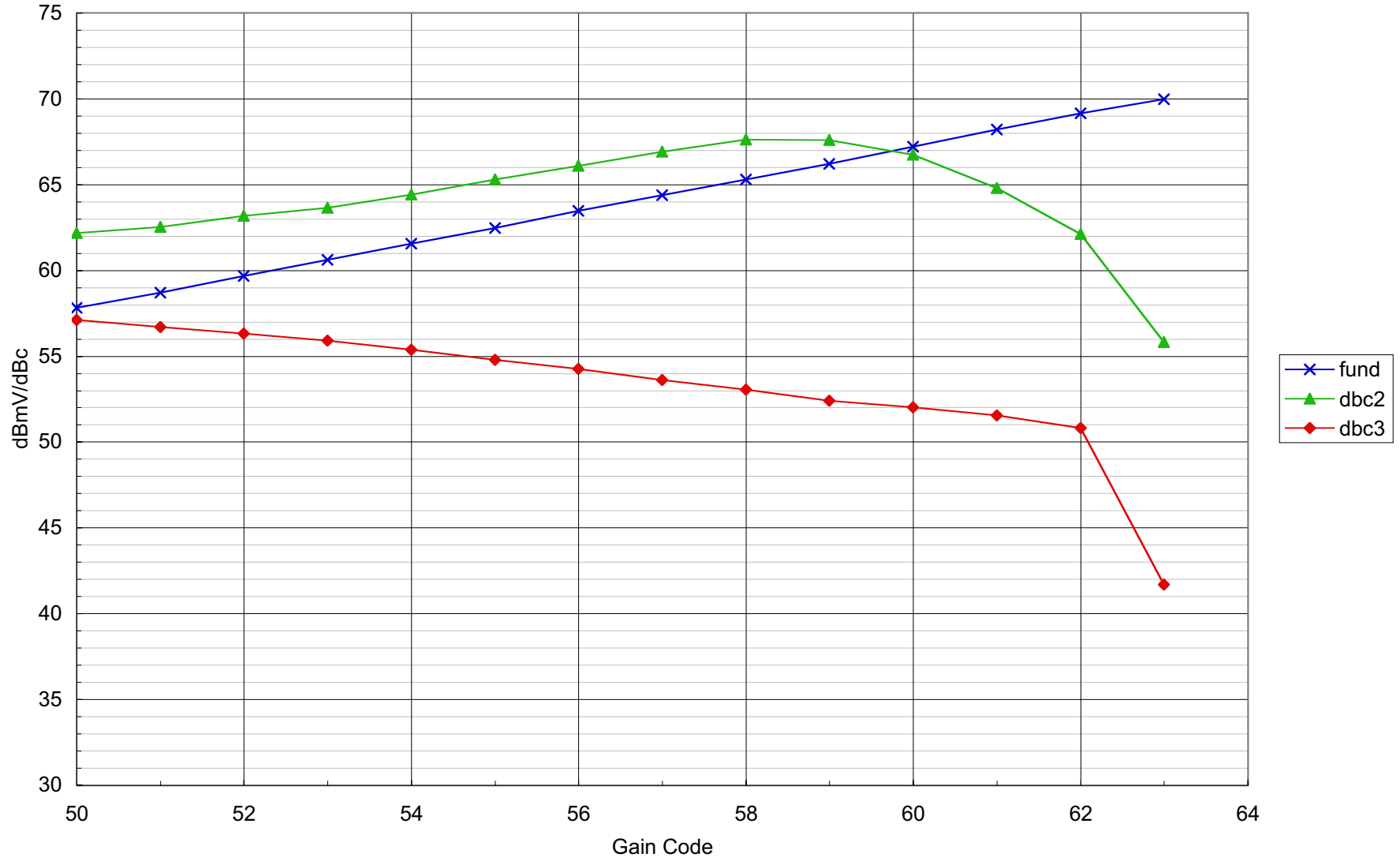
Pout, Harmonics vs. Gain Code MAX3509 22MHz 2:1 Pin=34dBmV
