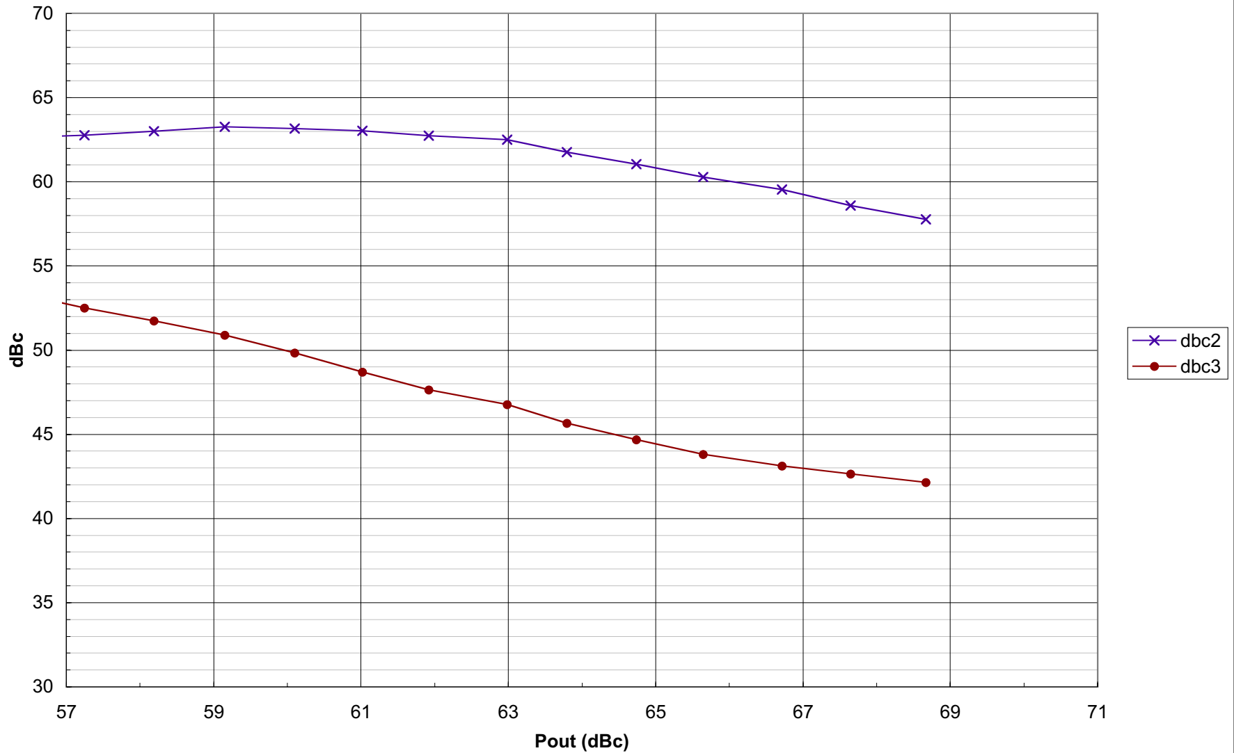
2nd 3rd Harmonic vs. Pout MAX3509 65MHz 2:1 Pin=33dBmV
