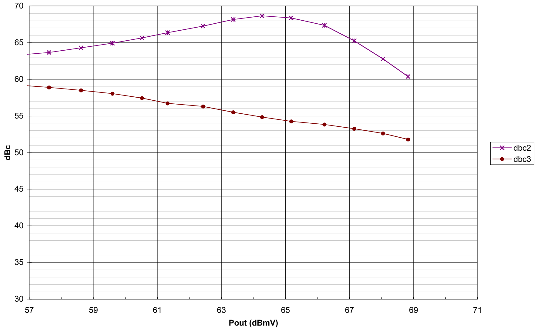
2nd 3rd Harmonic vs. Pout MAX3509 22MHz 2:1 Pin=33dBmV
