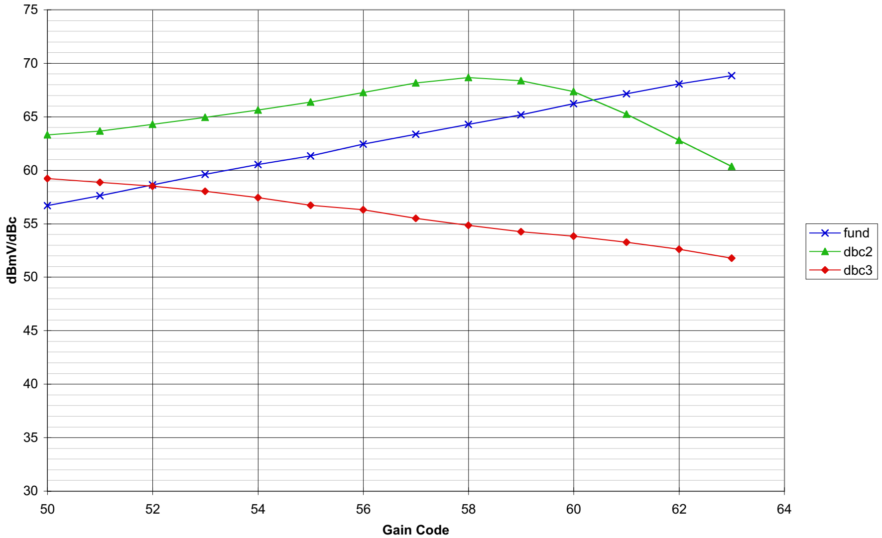
Pout, Harmonics vs Gain Code MAX3509 22MHz 2:1 Pin=33dBmV
