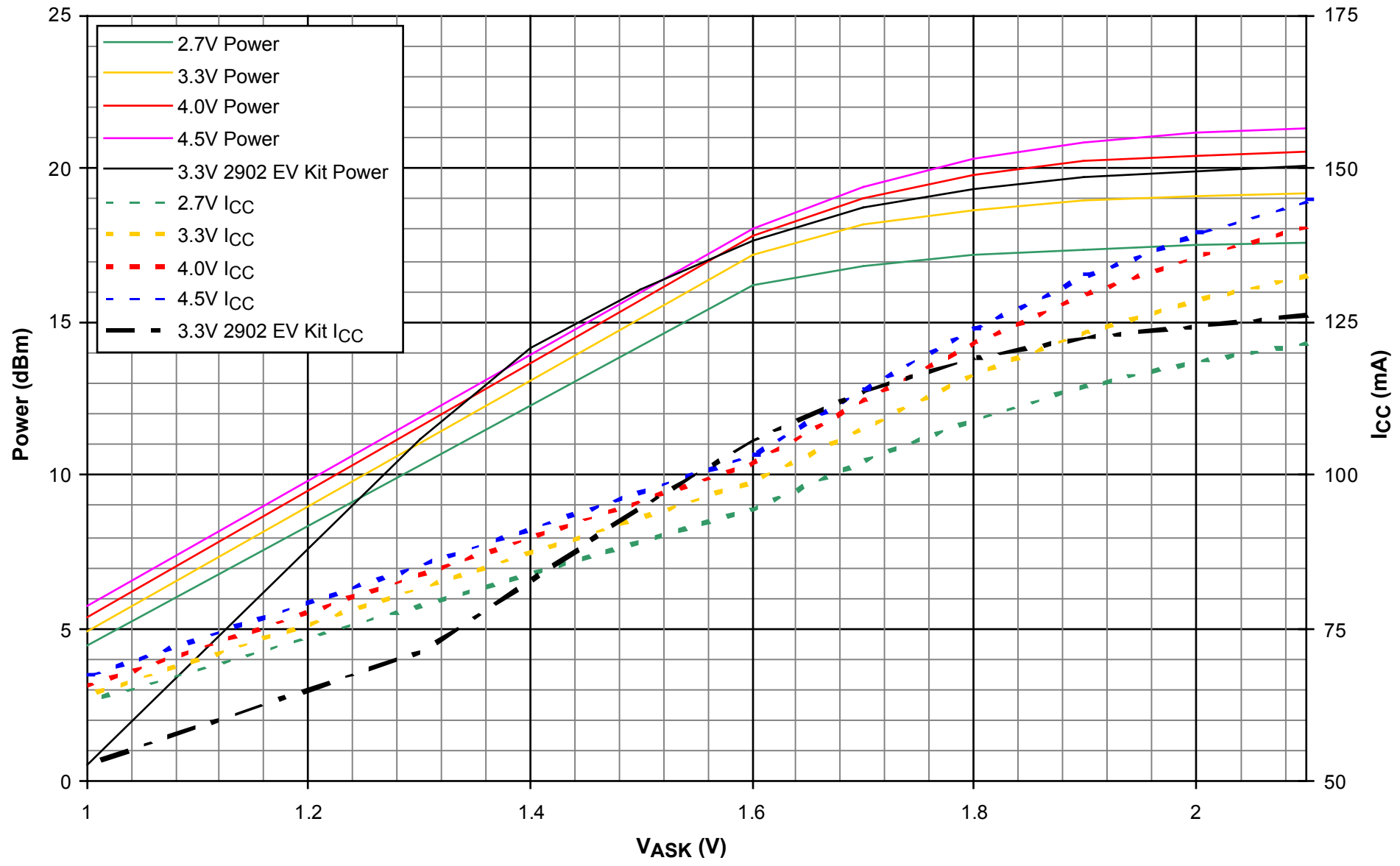
Power and I CC vs V CC 1:1 VSWR
